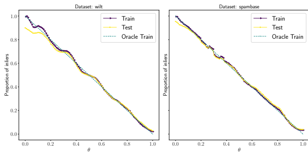
Figure 2: Density Level-Set Estimation: the \theta -property is approximately satisfied.
