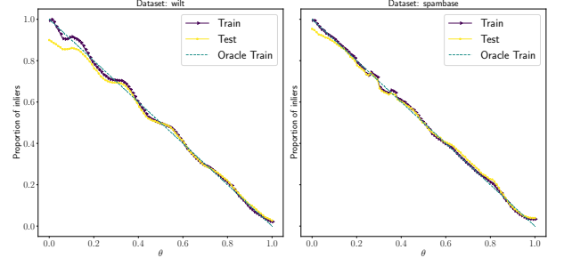
Figure 2: Density Level-Set Estimation: the \theta -property is approximately satisfied.
